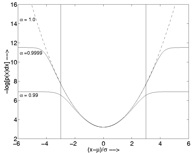
Figure 1: Contribution to local distance without (dashed line) and with (solid lines) acoustic backing-off for two different values of \alpha (i.e. 0.9999 and 0.99). Vertical lines indicate the boundaries of the region |\frac{x-\mu}{\sigma}| \leq 3 .
