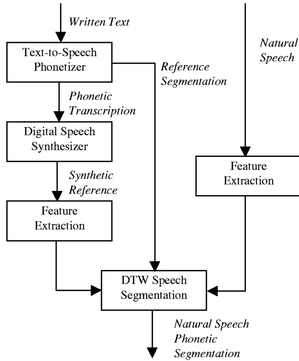
Figure 1 : Speech synthesis based alignment system.
