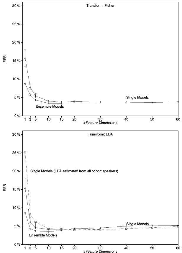
Figure 1: EERs for the Fisher and LDA based classifiers.
