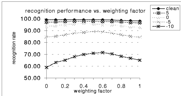
Fig. 4: Recognition rates at different SNRs for various values of the weighting factor \delta .
