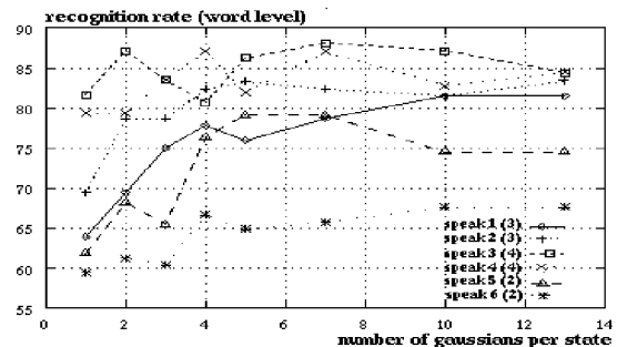
Figure 2: Word recognition rates measured for six speakers as a function of number of gaussians per state. The number in parentheses reports the speaker rate given by an expert.
