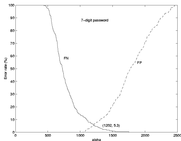
Figure 7. False-positive false-negative scores with 7-digit password
