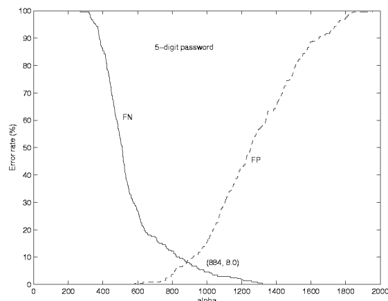
Figure 6. False-positive false-negative scores with 5-digit password
