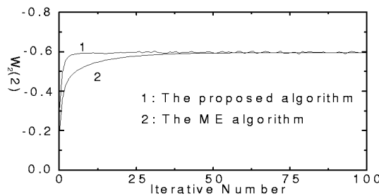
Figure 3: The convergent curves of weight W_2(2) .
