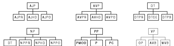
Figure 3: The ICE phrase-internal structures.
