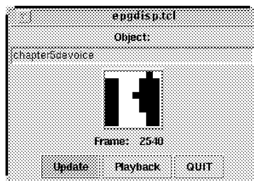
Fig 1. Devoiced /i/
