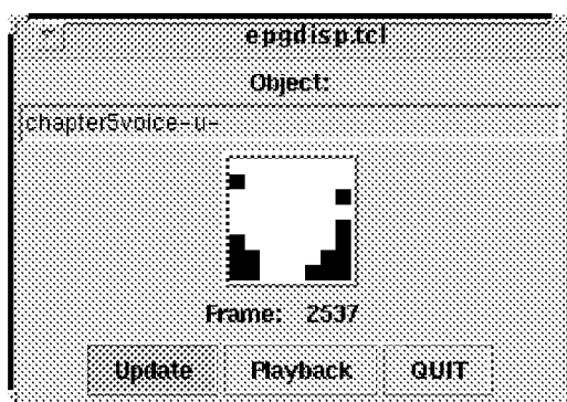
Fig 4. Voiced /u/
