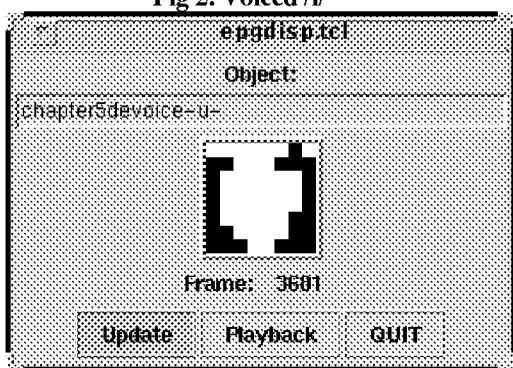
Fig 3. Devoiced /u/
