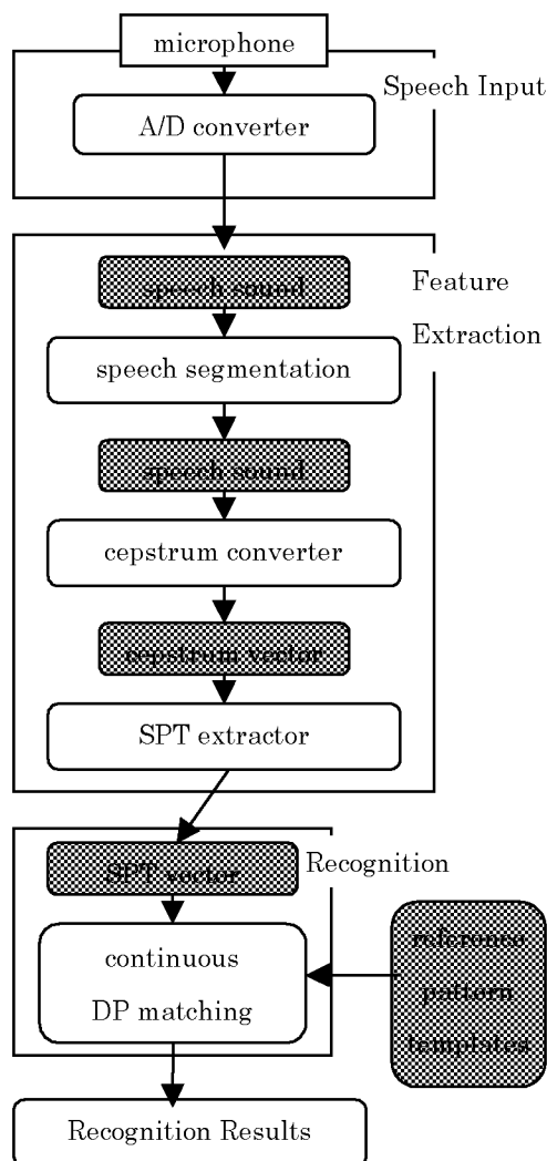
Fig.1 SPT Word-Spotter
