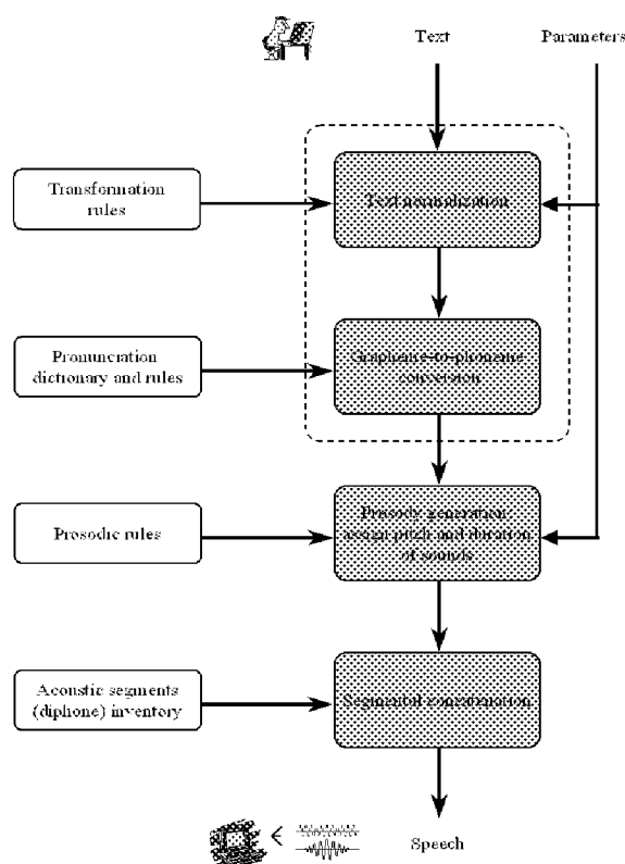
Figure 1: Slovene text-to-speech system.
