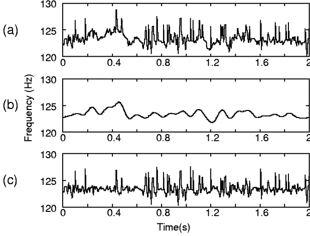
Fig. 4 Low- and high-pass filtered waves of the F0 wave shown in Fig. 3 (b): (a) original wave, (b) low-pass filtered wave, and (c) high-pass filtered wave with DC component.
