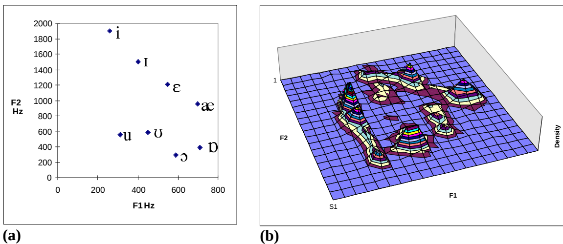
Figure 1: (a) The 'vowel space'. A formant chart showing the frequencies of the first and second formant for eight American English vowels. heed /i/, hid /I/, head /ε/, had /æ/, hod /ɒ/, hawed /ɔ/, hood /u/ and who'd /u/. (b) Three dimensional view of citation speech. A scatter plot of F1/F2 values from vowels in citation speech show how actual values produced relate to the vowel space. If the density of the scatter is plotted as a third dimension a 3d plot of the vowel space is produced. No scale is marked due to pre-processing.
