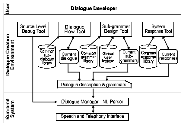
Figure 1: REWARD Platform architecture.
