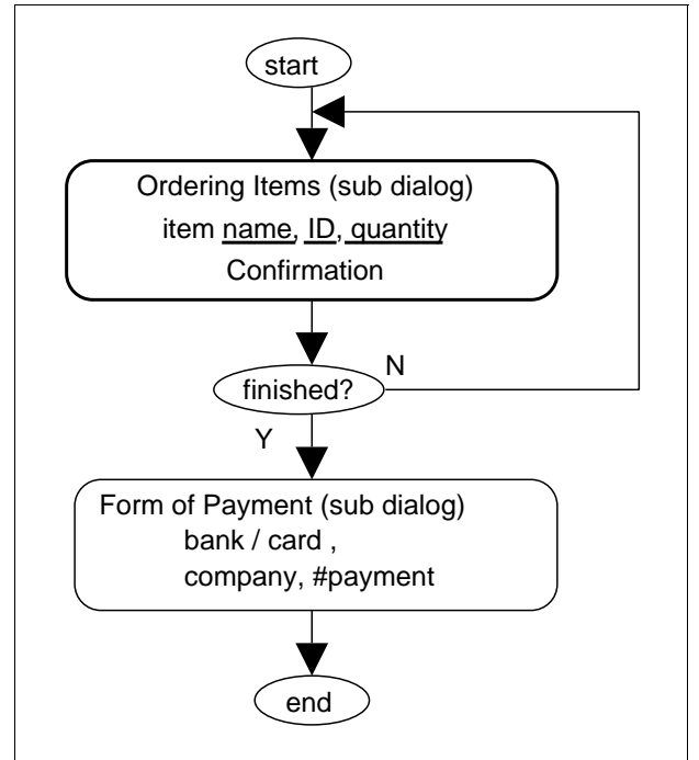
Figure 3: Dialogue flow
