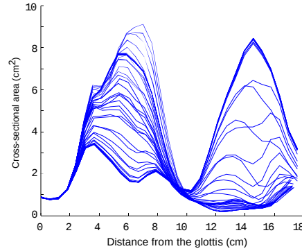
Fig. 6 Vocal tract area functions calculated from the physiological model for vowel sequence /iai/. Thin lines show the area functions during the transition between /i/ and /a/.
