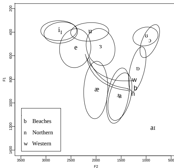
Figure 2: /ai/ trajectories for the three area groups superimposed on the monophthong target space.
