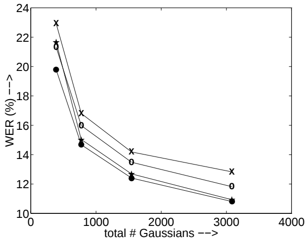
Figure 3: Recognition accuracy for cLR (x), pcR (*) and CMS (•), compared to the feature set without CN (o) when using CD-HMMs.
