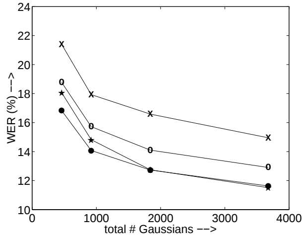
Figure 2: Recognition accuracy for cLR (x), pcR (*) and CMS (•), compared to the feature set without CN (o) when using CI-HMMs.
