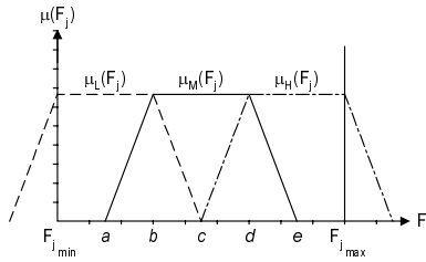
Figure 2: Trapezoidal Fuzzy Membership Function. [5]
