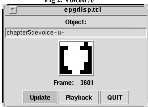
Fig 3. Devoiced /u/
