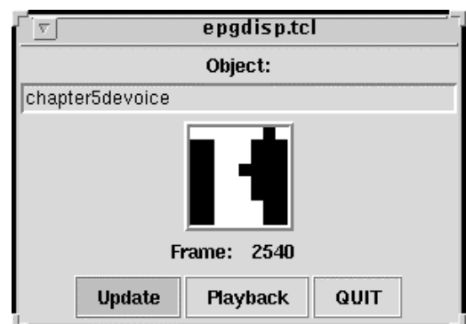
Fig 1. Devoiced /i/
