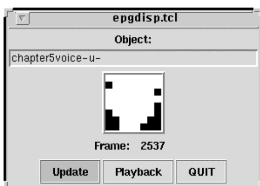
Fig 4. Voiced /u/
