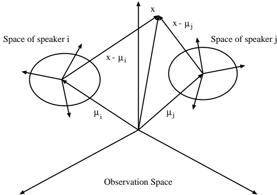
Figure 2: Speaker subspace
