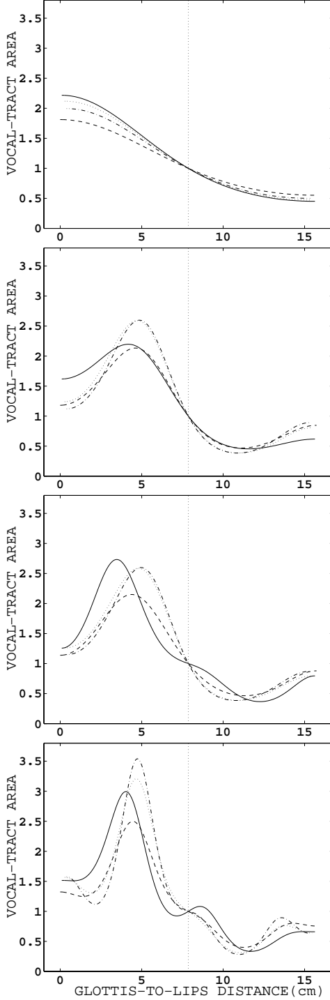
Figure 1: Multi-speaker, Vocal-Tract (VT) shapes estimated from \mathbf{F}_1 (top graph), \mathbf{F}_{12} (second from top graph), \mathbf{F}_{123} (third from top graph) and \mathbf{F}_{1234} (bottom graph) of one token of the (7-frame averaged) steady-state of the vowel in HEED . Four (4) speakers’ VT-shapes were first aligned at their respective mid-length, and then superimposed on each graph. Notation: \mathbf{F}_{12} \equiv \mathbf{F}_1\mathbf{F}_2 , and so on.
