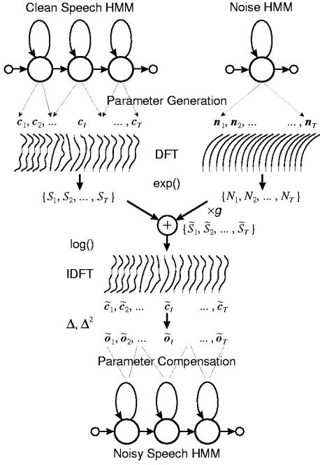
Figure 1: HMM-based parameter generation and compensation (PGC) [5].
