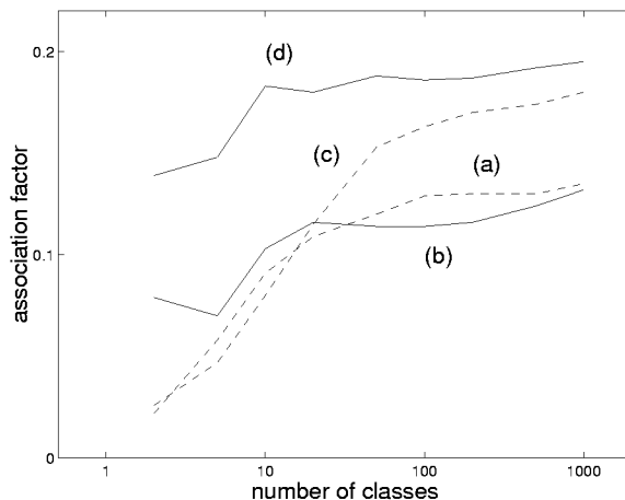
Figure 1. This figure shows strength of association between domains and classes for the following document space models; (a) unigram frequency/Euclidean norm, (b) unigram frequency/cosine angle, (c) inverse doc factor/Euclidean norm, and (d) inverse doc factor/cosine angle.
