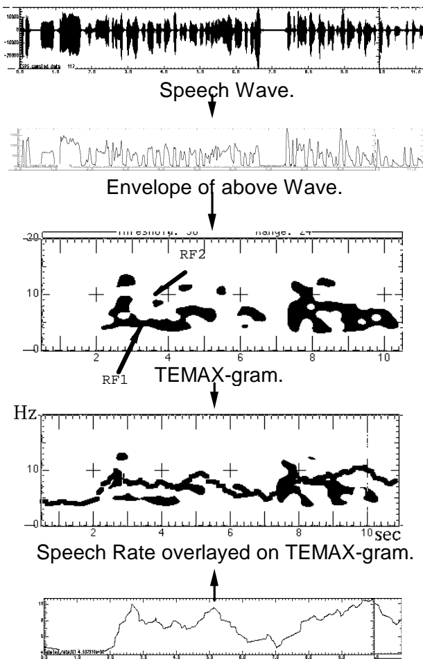
Speech Rate as Averaged Syllable Duration.
