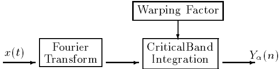
Figure 1: Speaker-specific Bark/Mel scale VTLN
