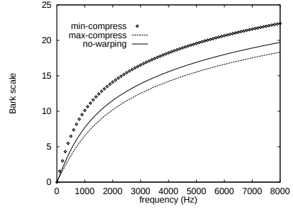
Figure 2: Bark scale warping curves
