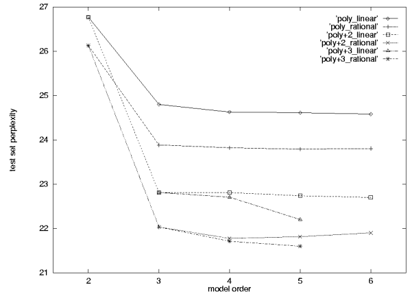
Figure 3. INTERCITY corpus
