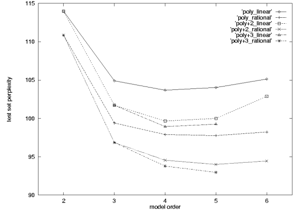
Figure 4. VERBMOBIL corpus
