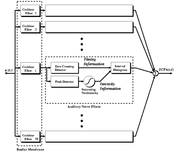
Figure 1: Block diagram of the zero-crossings with peak amplitudes (ZCPA) model.
