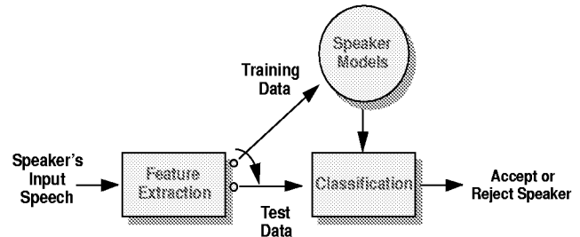
Figure 1: General speaker verification system
