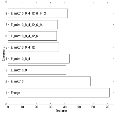
Figure 2: Distances for best feature sets of each search stage using development speaker set
