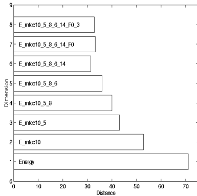
Figure 3: Distances for best feature sets of each search stage using test set
