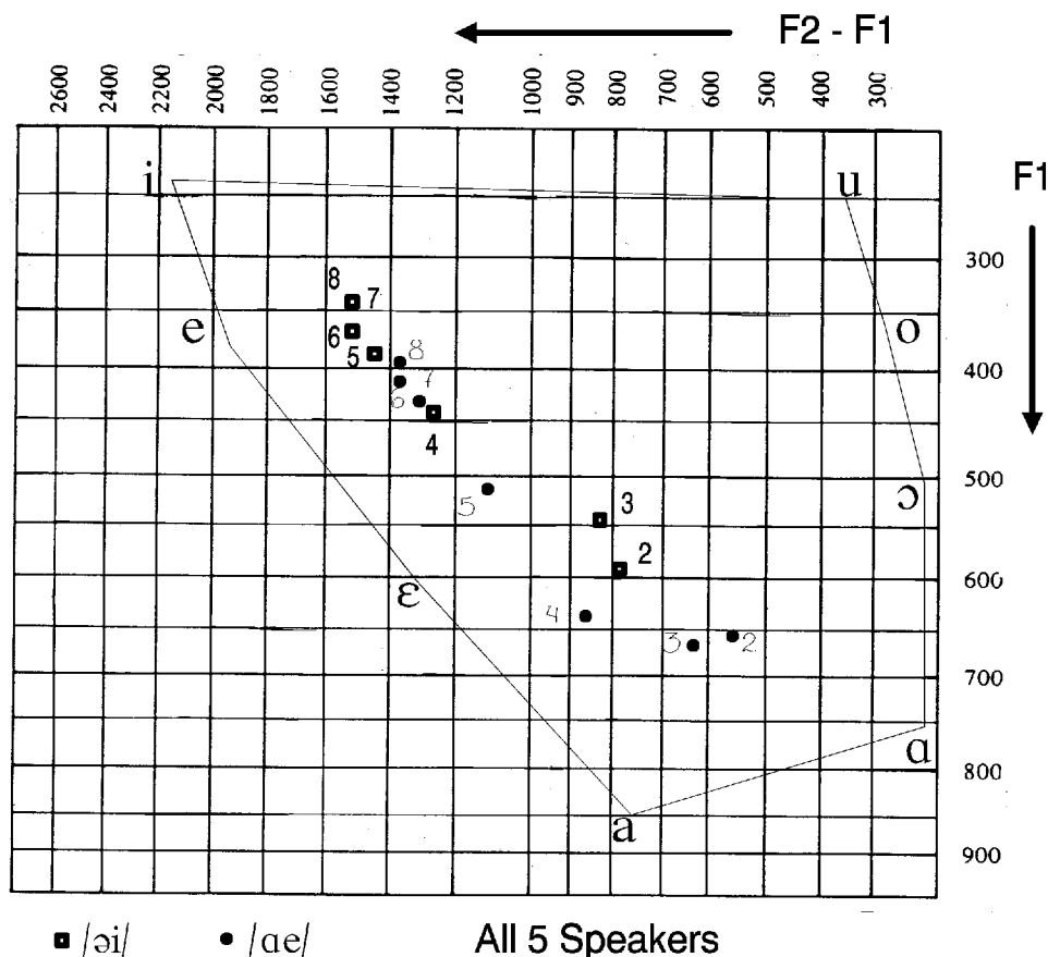
Figure 2. Trajectories of the diphthongs measured. The estimated values for cardinal vowels have been indicated. Formant values are given in [Hz].
