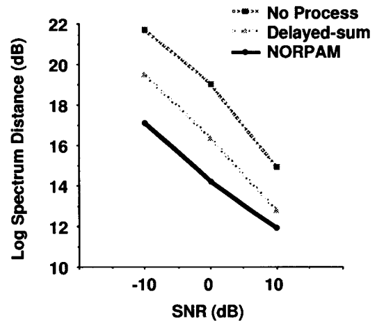
Fig. 7. Mean log-spectrum distances.
