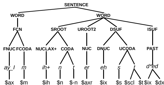
Figure 1: Sample parse tree for the phrase “I’m interested.” From top to bottom, the layers shown are: sentence, word, morphology, syllabification, phonemics, and phonetics.
