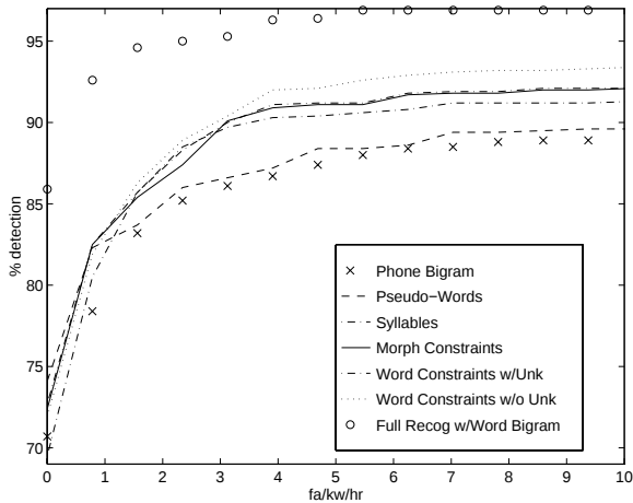
Figure 2: ROCs for various filler models.
