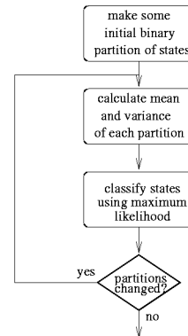
Figure 3: CPA-based partitioning
