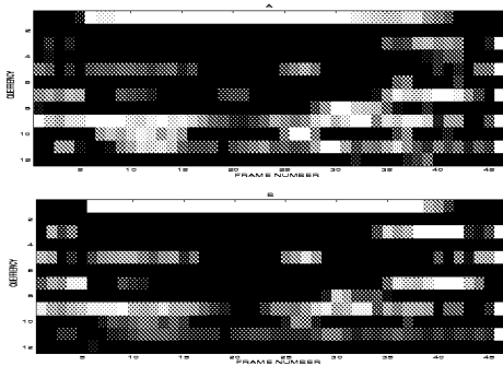
Figure 2: “Cepstrogram” for the utterance “four”: (A) original mel-based cepstrum before feature transformation, (B) after feature transformation.
