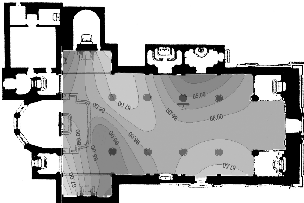
Figure 8 – Spatial distribution of L_{eq} Levels in post operam measurement session
