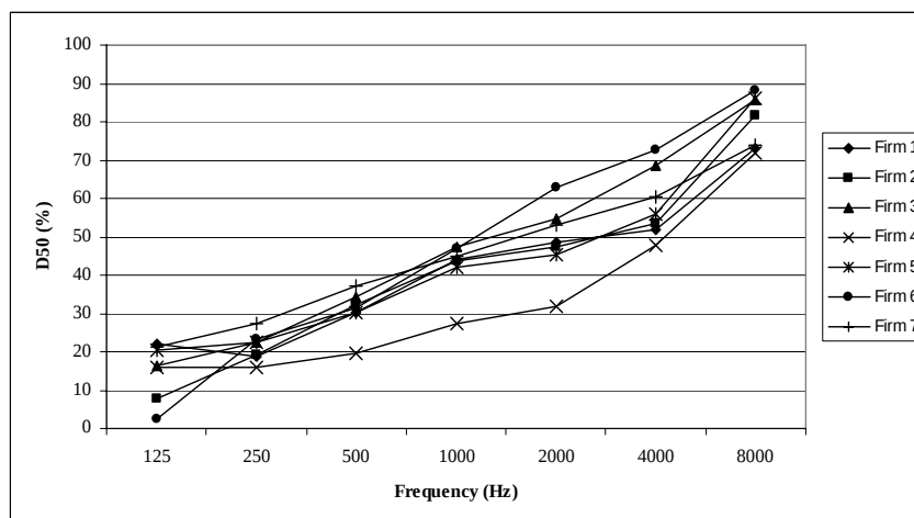
Figure 4 – Measured D_{50} values for the seven different electro-acoustic systems
