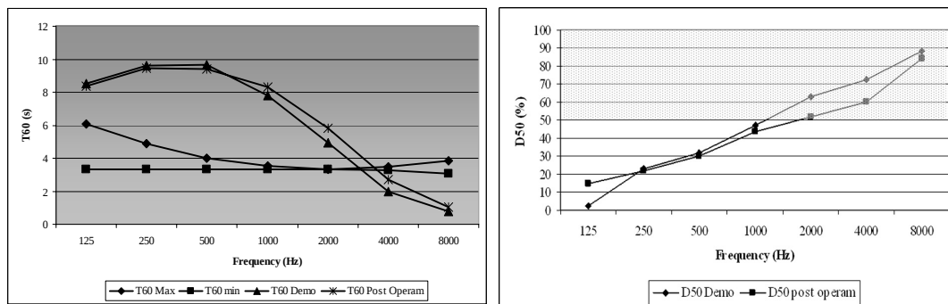
Figure 6 – Post operam results: T_{60} (left) and D_{50} (right) mean values and optimal range
