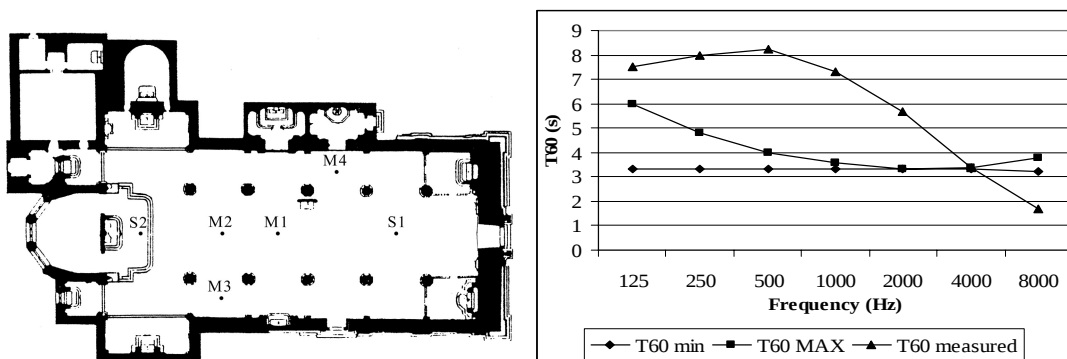
Figure 1 – (Left) San Lorenzo Cathedral's plan – Source (S1, S2) and microphone positions (M1 to M4). (Right) Reverberation Time measured and optimal range for the church
