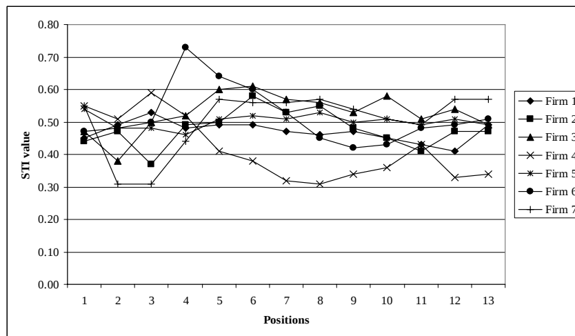
Figure 3 – Measured STI values for the seven different electro-acoustic systems
