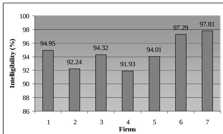
Figure 5 – ALCons test results for the seven different firms
