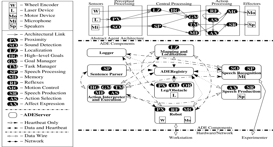
Figure 2: An overview of the DIARC architecture used for the team task components (top), its implementation in the ADE framework (middle), and mapping onto computing hardware (bottom). Boxes depict concurrently running components of varying complexity and arrows indicate the information flow through the architecture.
