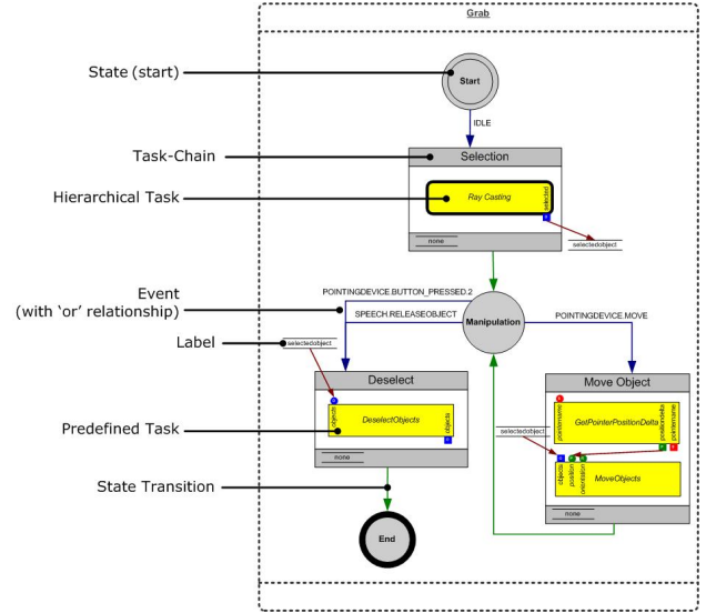
Figure 2: An Example of a NiMMiT diagram.
