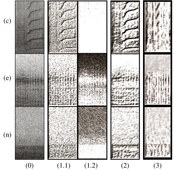
Fig. 3. Visualization of 3 samples of the call type dataset. From top to bottom: N9 call (c), echolocation (e), noise (n). From left to right: Input spectrogram (0), two of the strongest activations of the initial convolution layer (1.1, 1.2), one activation of the first ResNet layer (2) and one activation of the second ResNet layer (3). The activations in each column are the result of using exactly same convolutional kernel.
