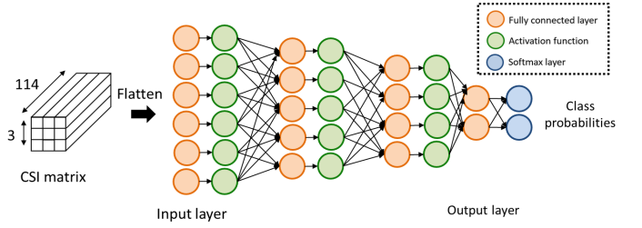
Fig. 6. Neural network architecture with two fully connected hidden layers and ReLU activation
