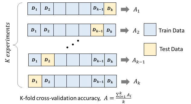
Fig. 4. k-fold validation technique
