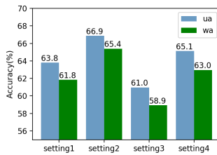
Fig. 5: The UA and WA on setting 1 ~ setting 4.
