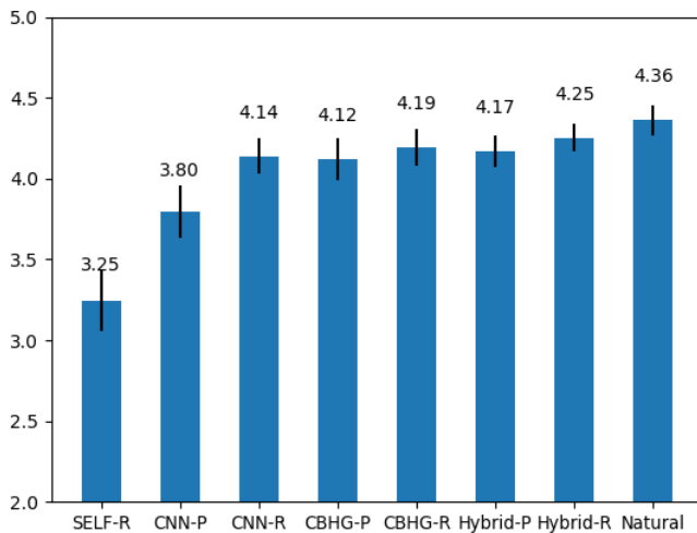
Fig. 3. MOS test results of various systems with 95% confidence intervals.
