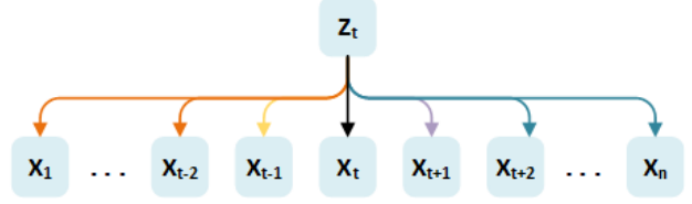
Fig. 2. Example relative edges representation with m = 2 . When generating z_t , there are n additional edges a_{tj}^K , where different colors represent different vectors. For j \leq t-2 or j \geq t+2 , the representation is clipped to the same \omega_{-2}^K and \omega_2^K , respectively.
