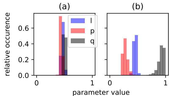
Fig. 2. Histogram of the parameter values of l , p and q from Equation 5 computed on the development set after joint training. (a) using the first-T frames noise estimator (b) using the mask based noise estimator
