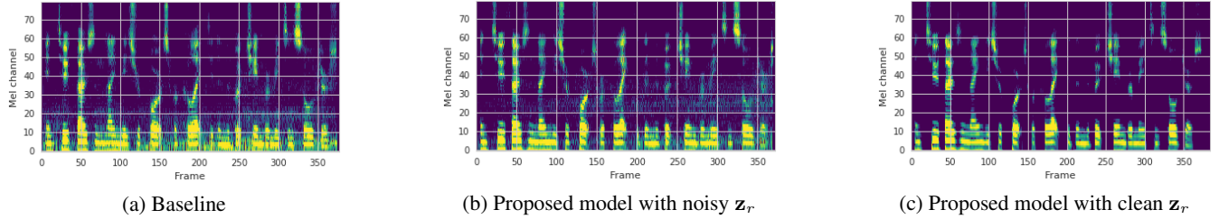
Fig. 2. Synthesized utterances of a noisy speaker (p252) from the baseline model (a), and our proposed model conditioning on \mathbf{z}_s inferred from a noisy utterance of p252, along with two \mathbf{z}_r from different speakers, one from a noisy utterance (b), and the other from a clean utterance (c).
