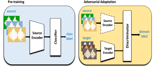
Fig. 2: Overview of the proposed Adversarial Discriminative Domain Adaptation (ADDA) approach. Source DNN encoder is fixed during the adversarial adaptation.
