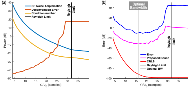
Fig. 3: In order to demonstrate our method of optimal bandwidth selection, we have generated synthetic signals using the ToF kernel, with K = 2 spikes separated by \Delta = 9.8 ns, and corrupted by bounded noise with SNR = 20 dB. (a) The curves corresponding to 1) \varepsilon_\Omega (red), the blowup of the deconvolution error (6), 2) the actual condition number \kappa^{(i)} (yellow) obtained from the Definition 2.1, and 3) the simplified bound G(\Omega) combining (11) and (12) (blue). (b) The actual error |t_{k,\Omega} - t_k| (blue), and the bound G(\Omega)\varepsilon_\Omega (magenta), obtained from multiplying the corresponding curves in (a). The Rayleigh threshold is approximately 32 samples. We can see that both the actual optimal bandwidth, and the predicted one, are pretty close to each other, and both of them are below the Rayleigh limit. For comparison, the CRLB for the parameter identification problem \hat{m}(n\omega_0) = \hat{\phi}(n\omega_0)\hat{s}(n\omega_0) + \hat{e}(n\omega_0) , with |n| \leq \Omega/\omega_0 and e(t) white Gaussian noise, is shown in red, and it is difficult to identify the optimal value of \Omega based on it alone. The divergence of CRLB from the actual error may be partly due to the fact that the noise covariance matrix of \hat{e}_\phi in (7) becomes badly conditioned for large \Omega , and matrix pencil being non-optimal in such a regime.
