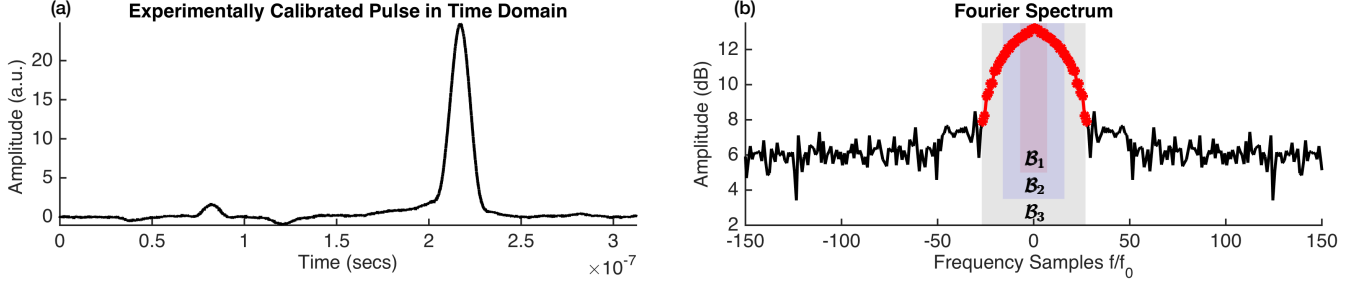
Fig. 1: (a) Time-domain samples of pulse \{\phi(nT)\}_{n=1}^{4464} calibrated using time-resolved sensor in [10]. Note that the pulse is smooth and asymmetric. (b) Fourier domain samples. Here \mathcal{B}_k = [-\Omega_k, \Omega_k] , k = 1, 2, 3 are possible bandwidths (for deconvolution) that can be used for super-resolving spikes.
