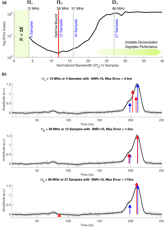
Fig. 2: Super-resolution is sensitive to bandwidth selection. (a) Estimation error as a function of bandwidth \Omega . Let \tilde{t}_{k,\Omega} be the estimated spike support for a given \Omega . The metric for error is chosen to be \max |\tilde{t}_{k,\Omega} - t_k| where t_k is the ground truth and the spikes are separated by \Delta = |t_2 - t_1| = 12.6 ns. Given noisy measurements m(t) (5) corrupted by 15 dB additive white Gaussian noise, this plot is obtained by sweeping bandwidth \Omega in the range \omega_0 \in [2K, N] and averaged over 200 realizations. The optimal bandwidth in this case amounts minimum value of the error curve. (b) Corresponding reconstruction for three scenarios: (1) Critical sampling with \Omega_1/\omega_0 = 2K . Here, the reconstruction fails because of noise. (2) Optimal \Omega_2 obtained by sweeping \Omega and observing the minimum of the error in (a). This scheme benefits from over-sampling. (3) Excessive over-sampling when \Omega_3 approaches the noise floor. Here reconstruction fails because unstable deconvolution leads to erroneous estimates of sinusoidal parameters in (3). We use matrix pencil method [11] for frequency estimation.
