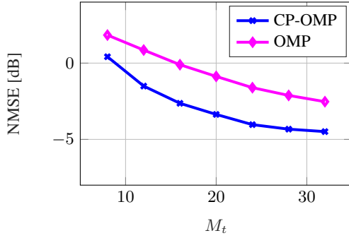
Fig. 3. NMSE vs. M_t . SNR = 0 dB.
