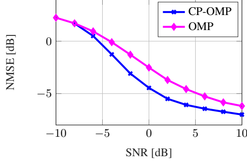
Fig. 2. NMSE vs. SNR. M_t = 32 transmissions.
