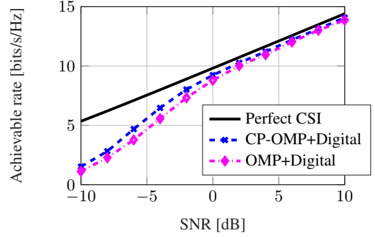
Fig. 4. Achievable rate vs. SNR. M_t = 32 transmissions.
