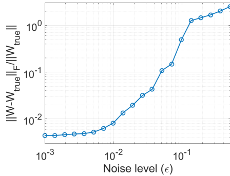
Fig. 3. Evolution of the recovery of the true W depending on the noise N = \epsilon \text{ rand}(m, n) using Alg. 1 ( \tilde{\lambda} = 0.01 , \delta = 0.1 , \text{maxiter} = 100 ).
