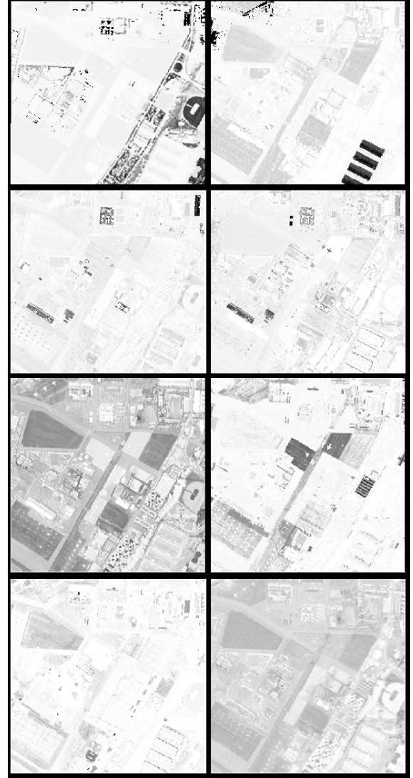
Fig. 4. Abundance maps extract by min-vol NMF using only five bands of the San Diego airport HSI. From left to right, top to bottom: vegetation (grass and trees), three different types of roof tops, four different types of road surfaces.
