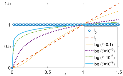
Fig. 1. Function \frac{\log(x^2 + \delta) - \log(\delta)}{\log(1 + \delta) - \log(\delta)} for different values of \delta , \ell_1 norm ( = |x| ) and \ell_0 norm ( = 0 for x = 0 , = 1 otherwise).
