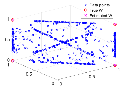
Fig. 2. Synthetic data set and recovery. (Only the first three entries of each four-dimensional vector are displayed.)
