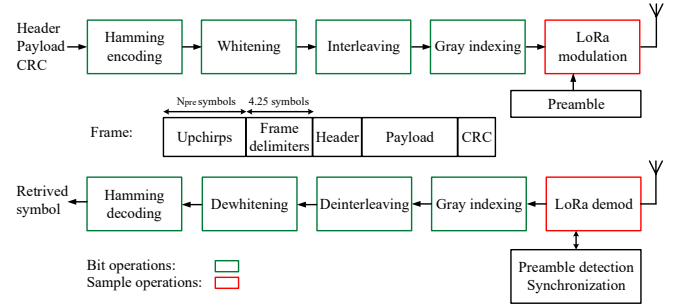
Fig. 1: LoRa frame structure [4] and PHY block diagram.
