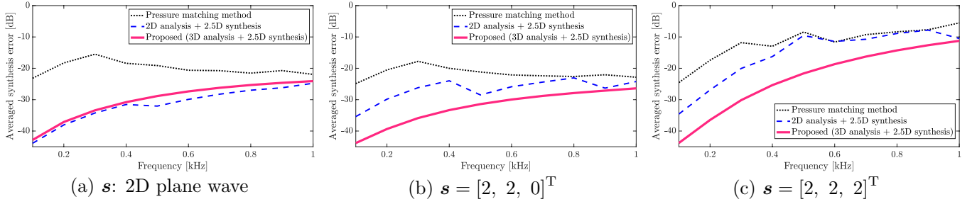
Fig. 3. Results of averaged synthesis error in horizontal plane for r \leq 0.2 m and 100 \text{ Hz} \leq f \leq 1 \text{ kHz} : (a) primary recording sound field is 2D plane wave; (b) source position in primary sound field is \mathbf{s} = [2, 2, 0]^T ; (c) source position in primary sound field is \mathbf{s} = [2, 2, 2]^T .
