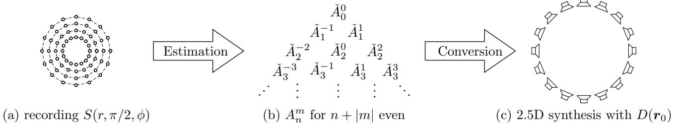
Fig. 1. Processing flowchart of proposed horizontal 3D sound field recording and 2.5D synthesis scheme: (a) recording horizontal 3D sound field S(r, \pi/2, \phi) with multiple co-centered omni-directional circular arrays; (b) estimating spherical harmonic spectrums A_n^m for n + |m| even from recorded horizontal sound pressures; (c) converting estimated spherical harmonic spectrums into driving function D(\mathbf{r}_0) and synthesizing horizontal 3D sound field with a circular loudspeaker array based on 2.5D higher-order Ambisonics.
