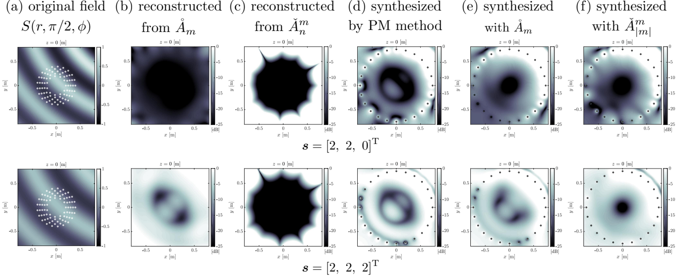
Fig. 2. Results of (a) original sound field; (b)-(f) reconstruction and synthesis errors in horizontal plane for two primary sound source locations of \mathbf{s} = [2, 2, 0]^T and [2, 2, 2]^T and frequency f = 500 Hz (b) reconstructed from estimated \hat{A}_m ; (c) reconstructed from estimated \hat{A}_n^m ; (d) synthesized by pressure matching (PM) method; (e) synthesized by 2.5D HOA for 2D sound field \hat{A}_m ; (f) synthesized by 2.5D HOA for horizontal 3D sound field \hat{A}_m^m . White circles in (a) and black circles in (d)-(f) represent microphones and loudspeakers, respectively.
