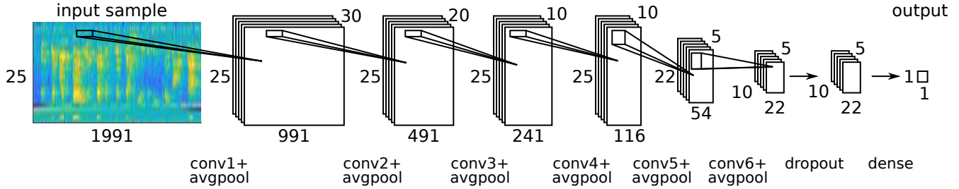
Fig. 2. CNN architecture used. The dropout layer rate was 50%, followed by a fully connected layer with one output node.
